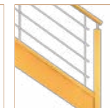
NIRTA R41 CROISÉS INOX Ø 12 MM
