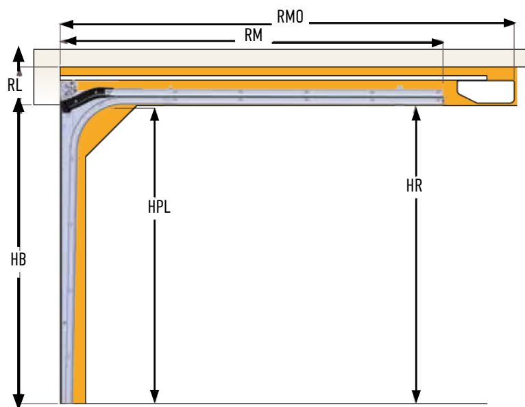
Linteau standard DUO 160
